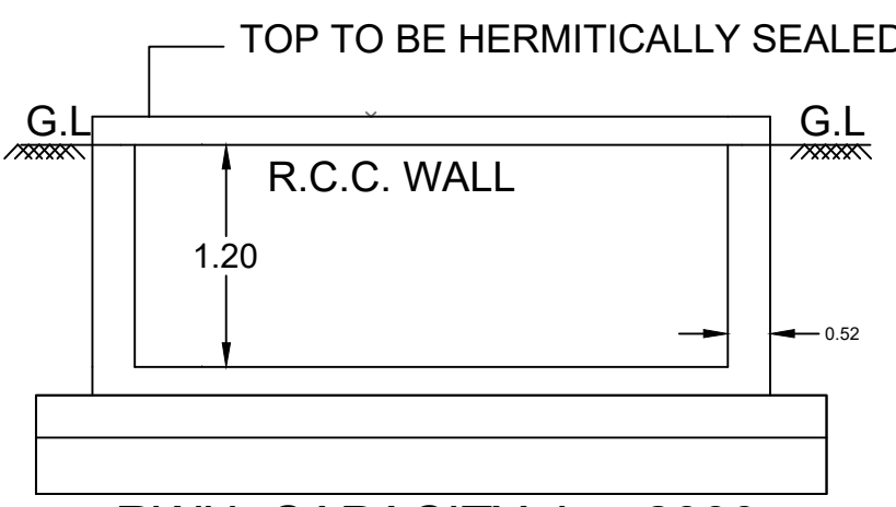
RWH_SECTION RWH_CAPACITY_L = 2000
