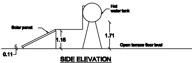
SIDE ELEVATION
