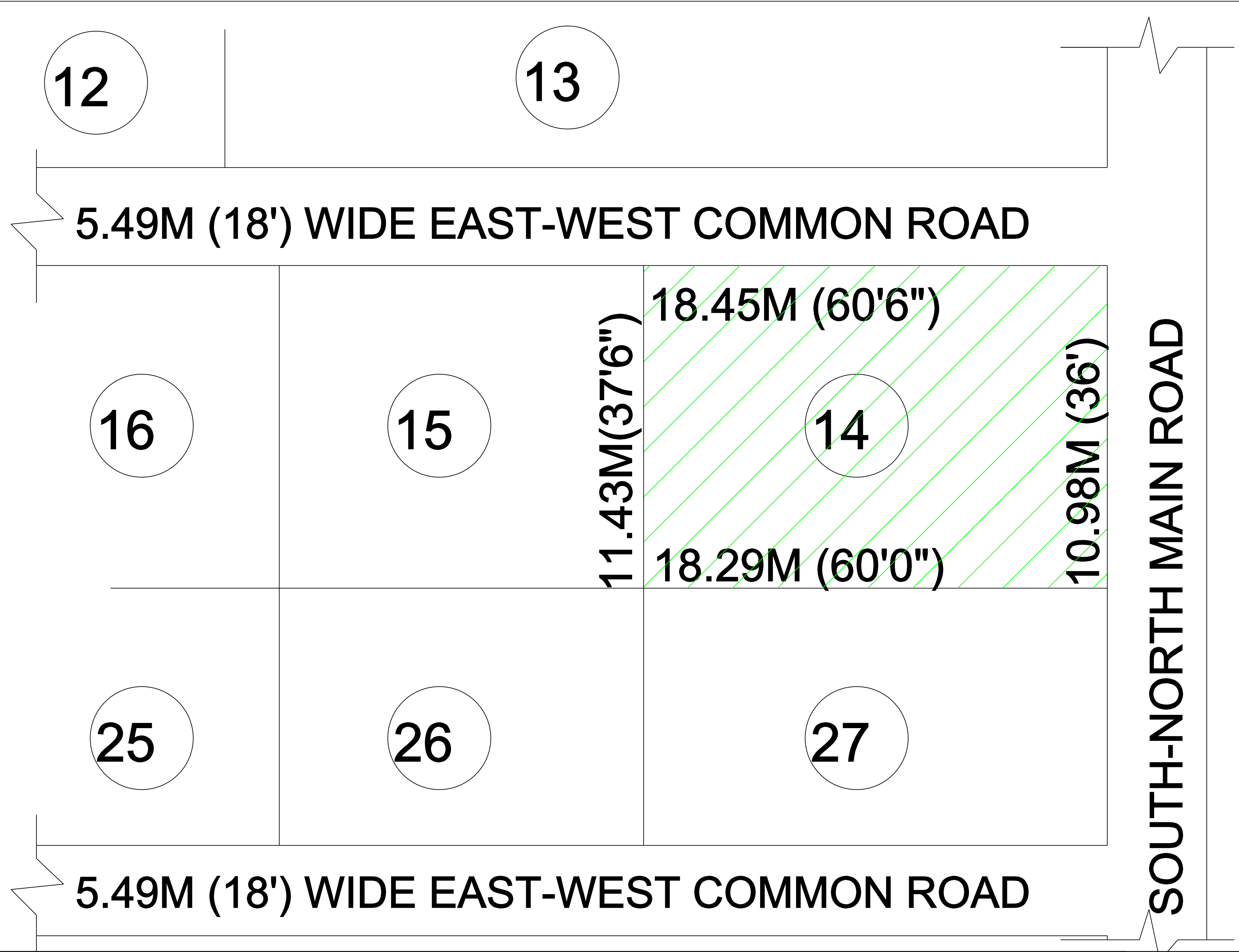
LOCATION PLAN
