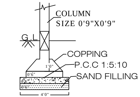
FOUNDATION DETAILS SCALE 1:50
