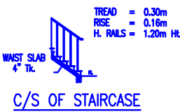
C/S OF STAIRCASE
