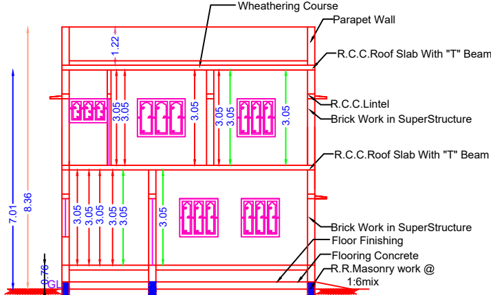
SECTION ON "PQ" SCALE 1:100
