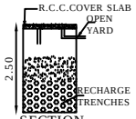
SECTION
