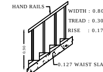
STAIRCASE DETAILS:-
