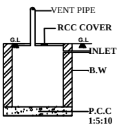
SEPTIC TANK
