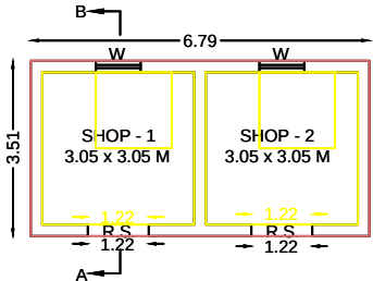
PROPOSED GROUND FLOOR PLAN
