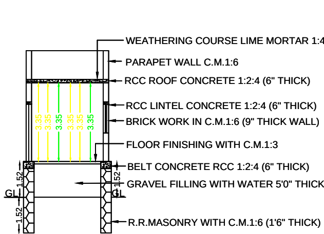
SECTION ON AB & CD
