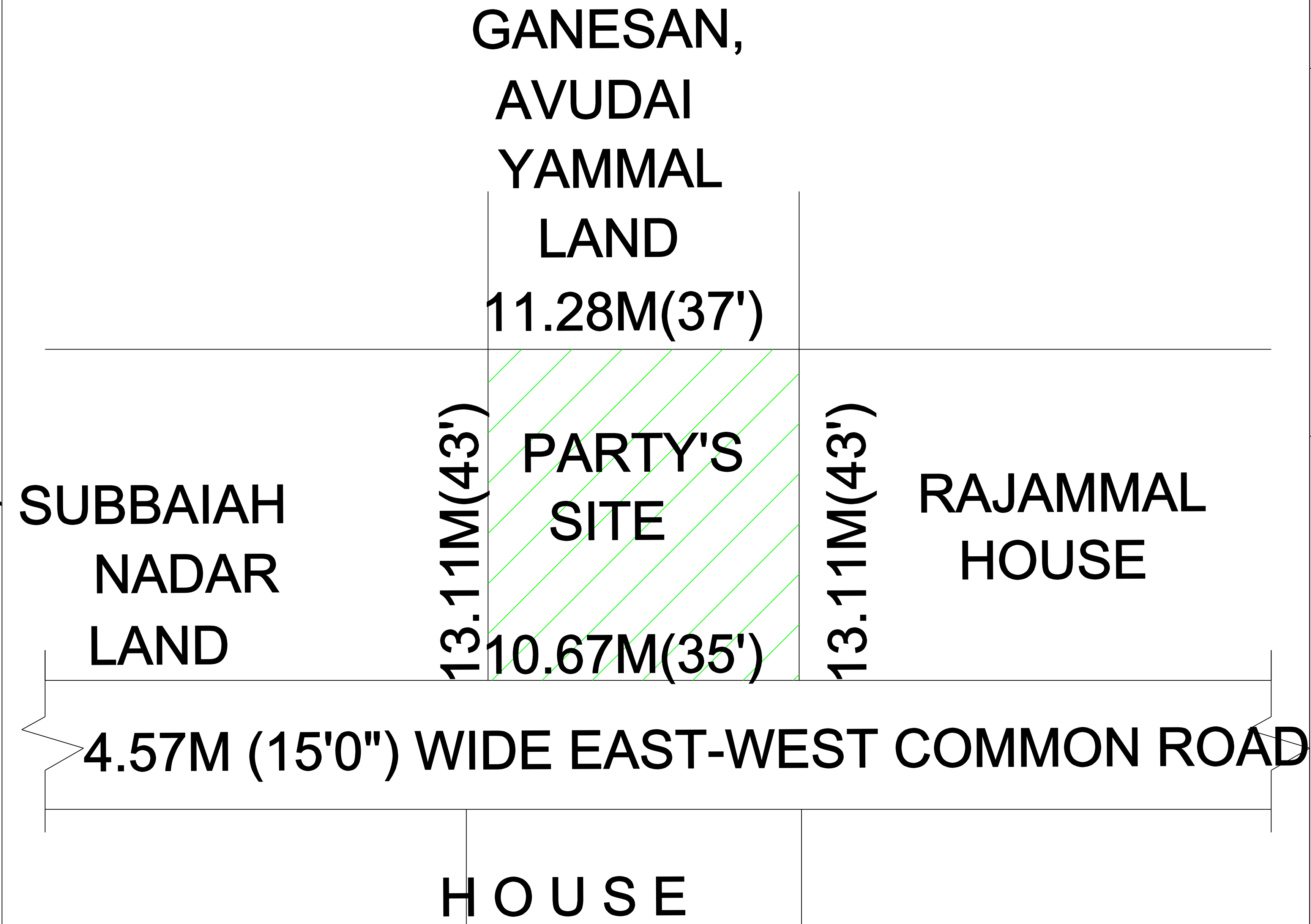
LOCATION PLAN
