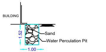
DETAILS OF RAIN WATER PERCOLATION PIT (SCALE 1:100)
