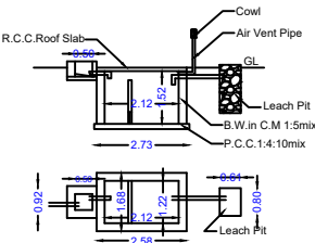
DETAILS OF SEPTIC TANK
