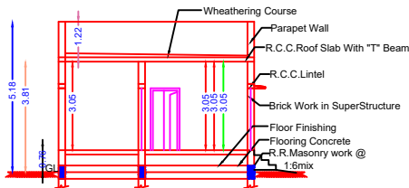
SECTION ON "PQ"
