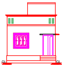
FRONT ELEVATION
