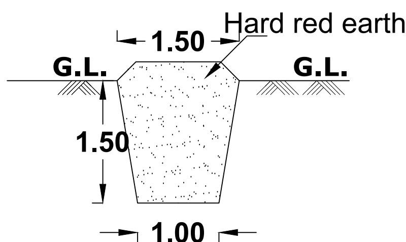
TRIAL PIT (Scale 1:100)
