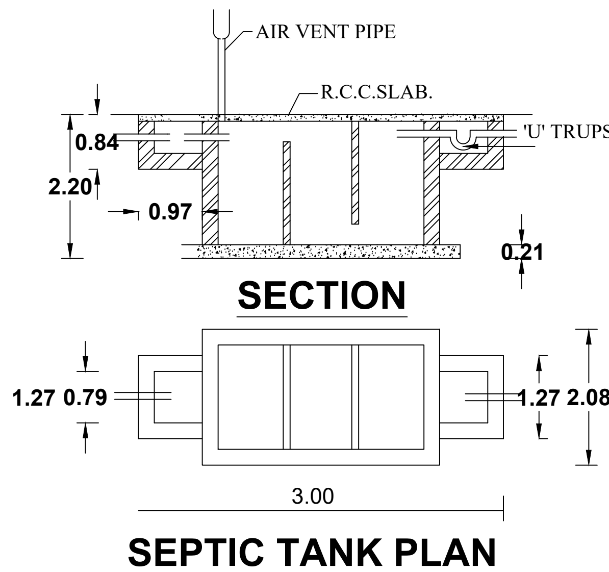
SEPTIC TANK PLAN
