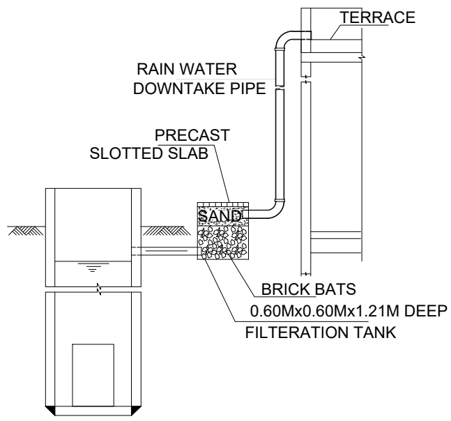
RAIN WATER HARVESTING SYSTEM
