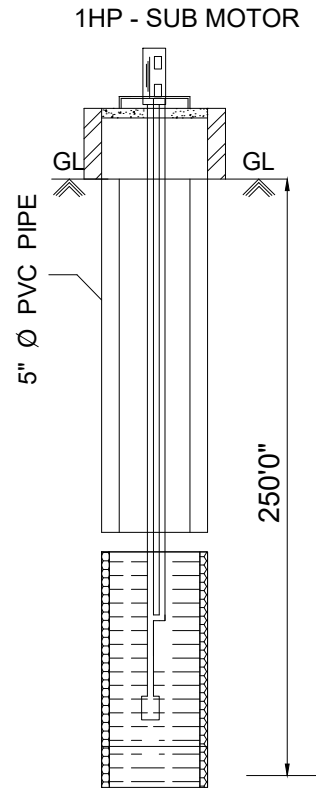
BOREWELL DETAILS
