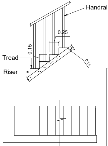
STAIRCASE DETAIL
