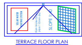
TERRACE FLOOR PLAN
