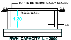
RWH SECTION
