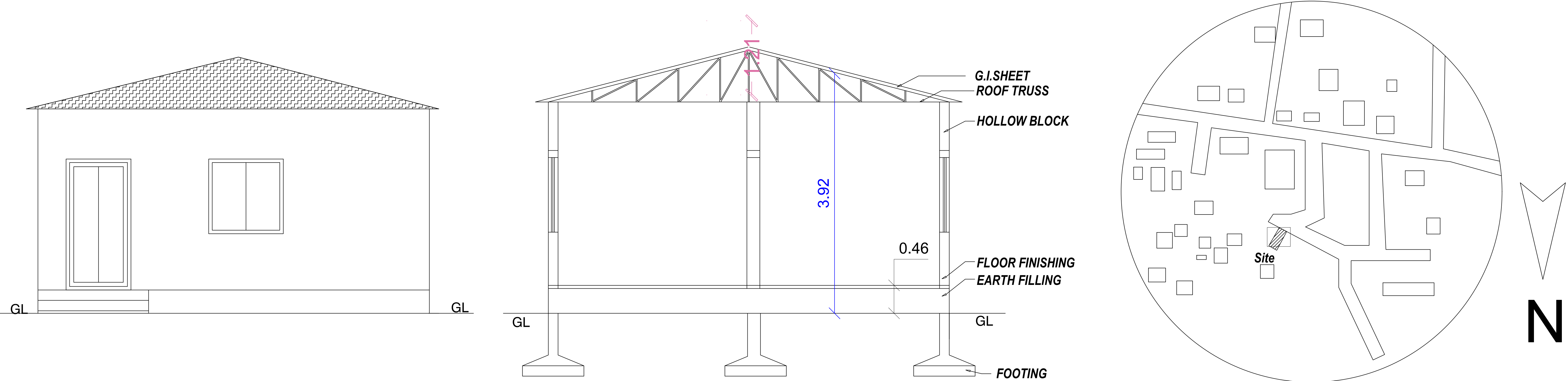
FRONT ELEVATION
