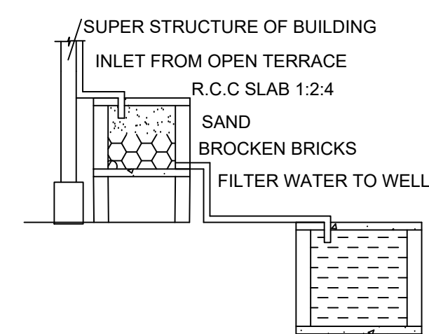
RAINWATER HARVESTING
