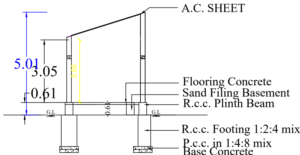
SECTION -"AB"
