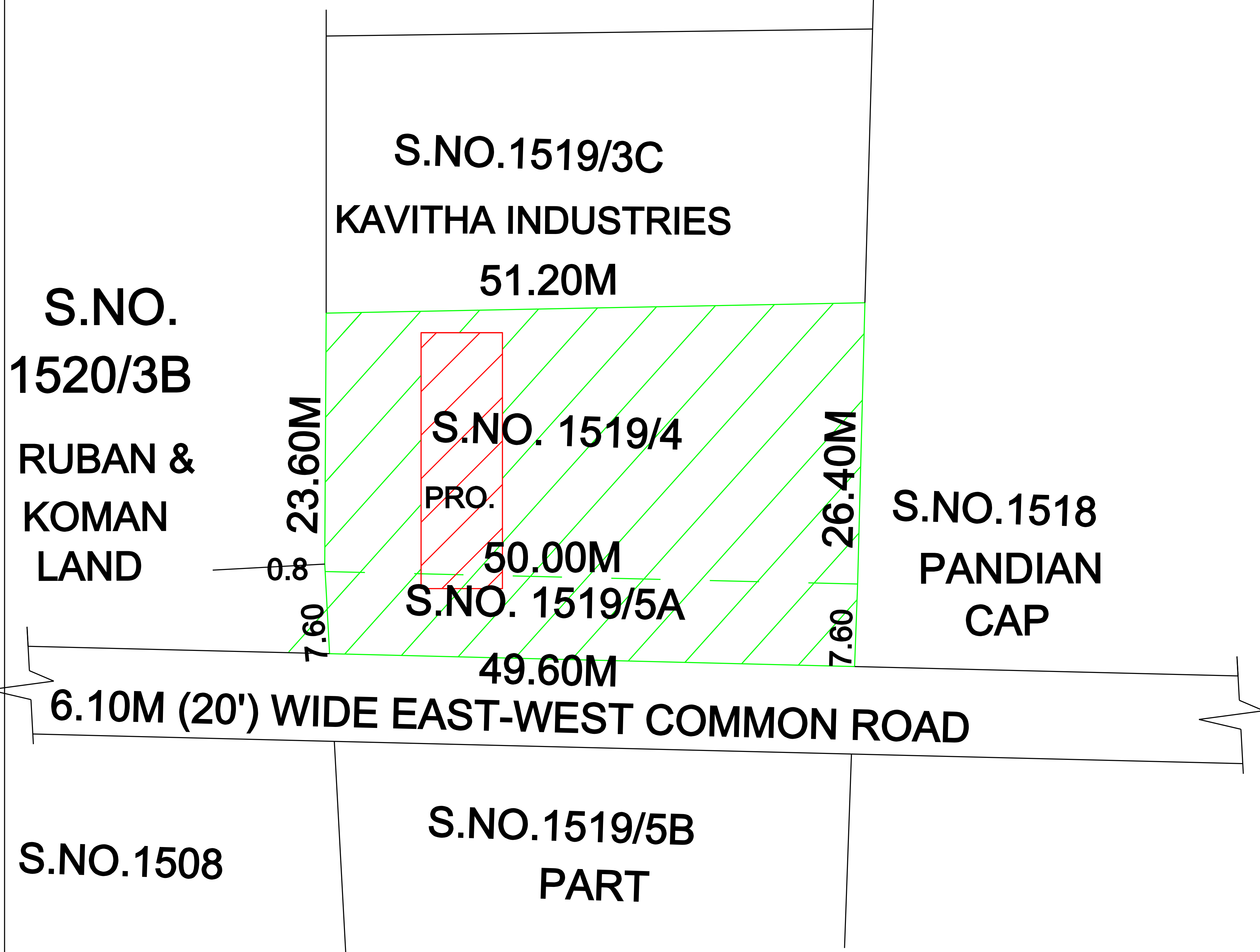
LOCATION PLAN
