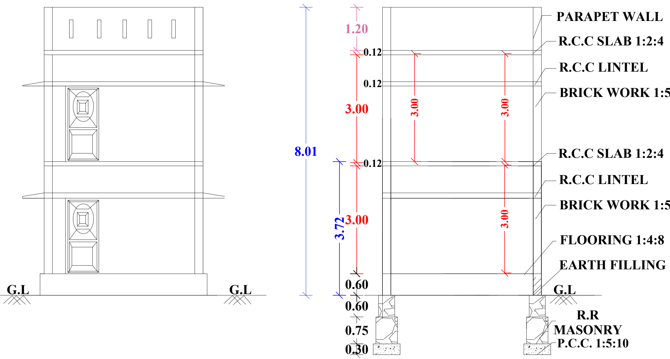
FRONT ELEVATION
