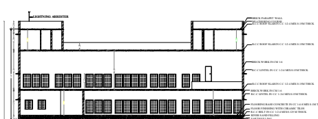
SECTION ON 'AA'
