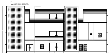
FRONT ELEVATION
