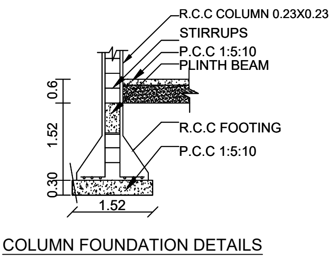
COLUMN FOUNDATION DETAILS
