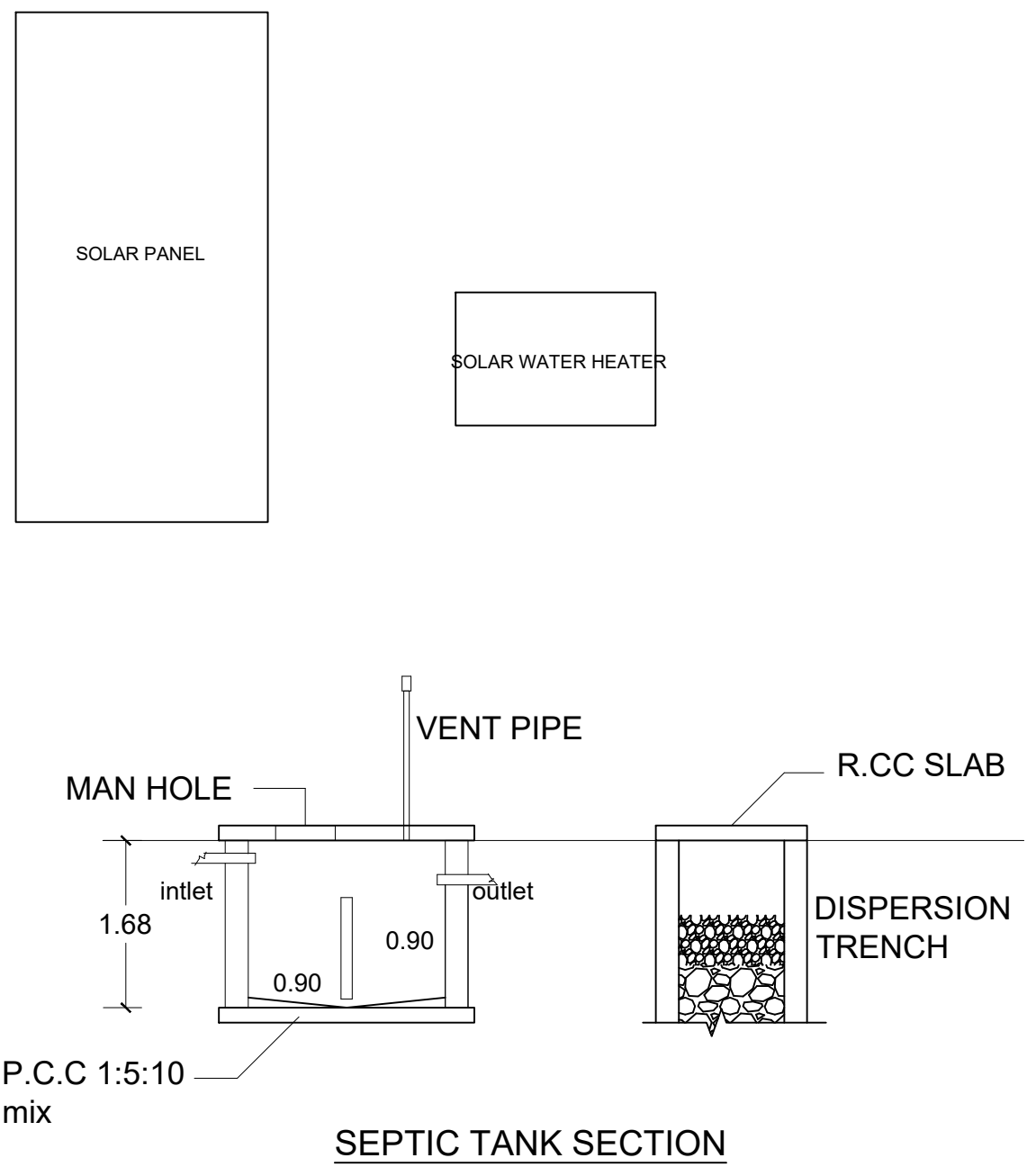
SEPTIC TANK SECTION
