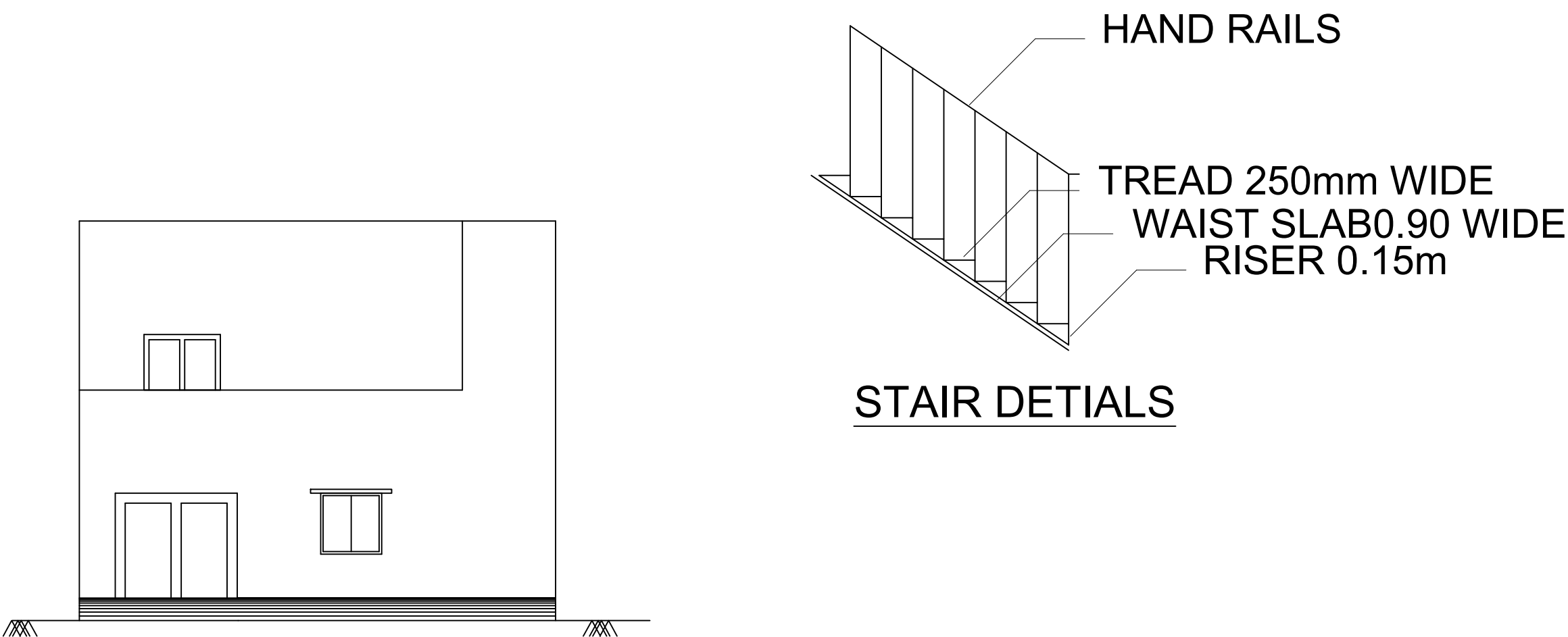
FRONT ELEVATION
