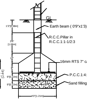
FOUNDATION DETAILS
