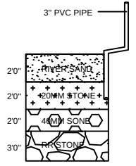
RAIN WATER HARVESTING
