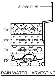
RAIN WATER HARVESTING
