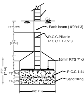
FOUNDATION DETAILS
