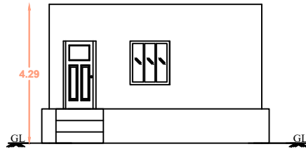
FRONT ELEVATION
