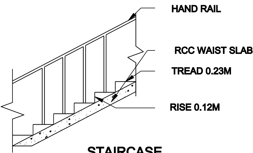
STAIRCASE
