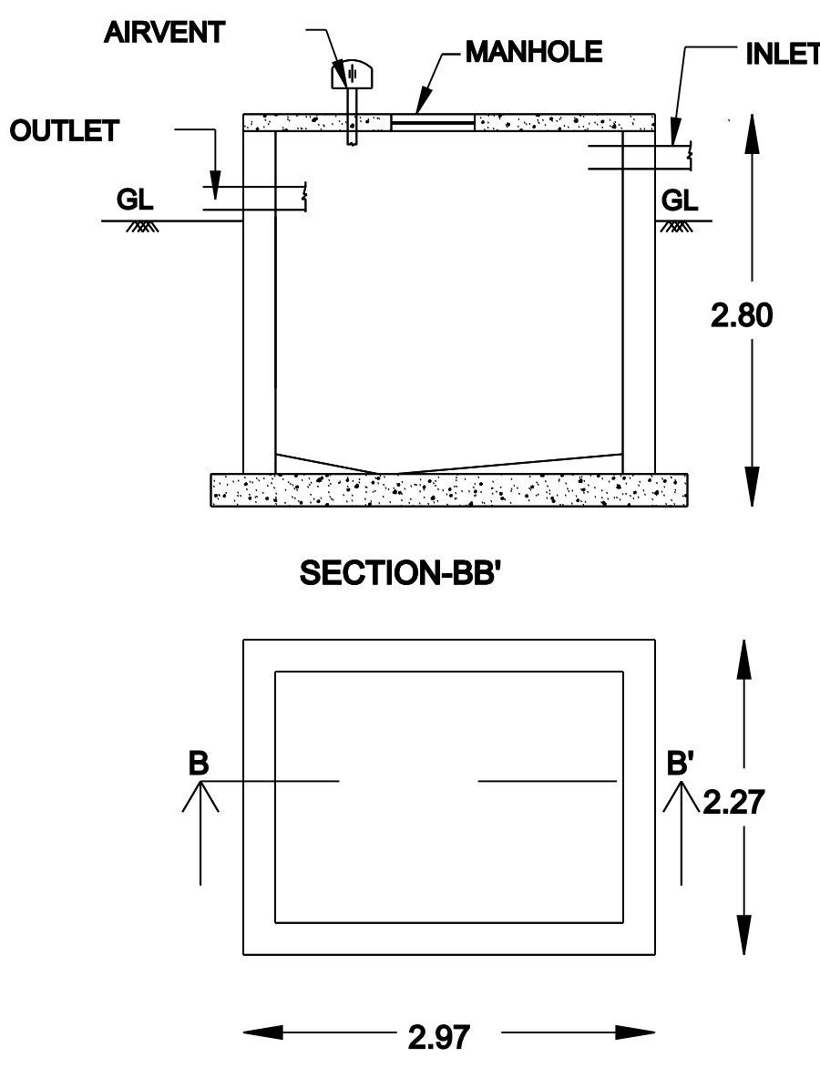
SEPTIC TANK
