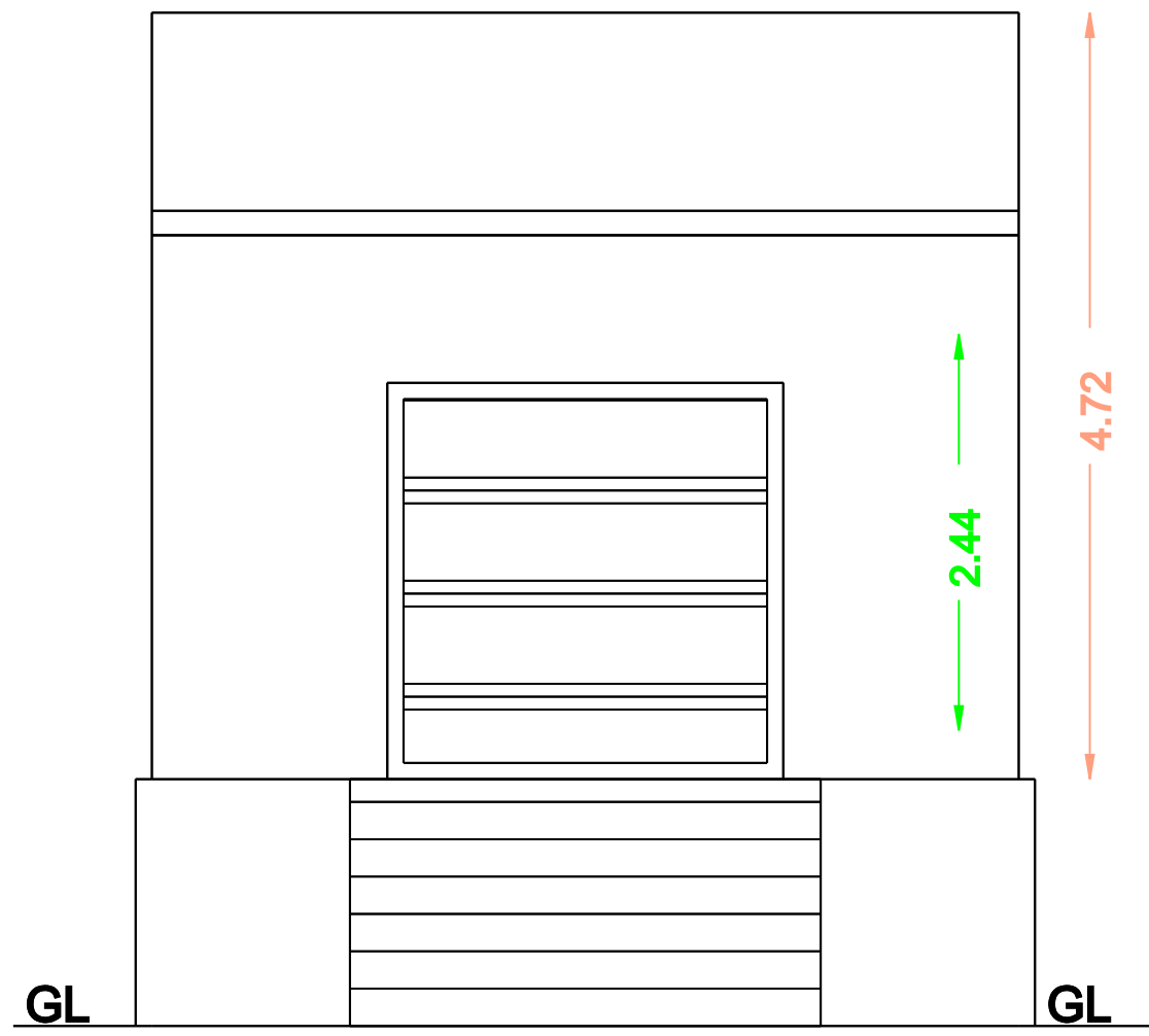
FRONT ELEVATION
