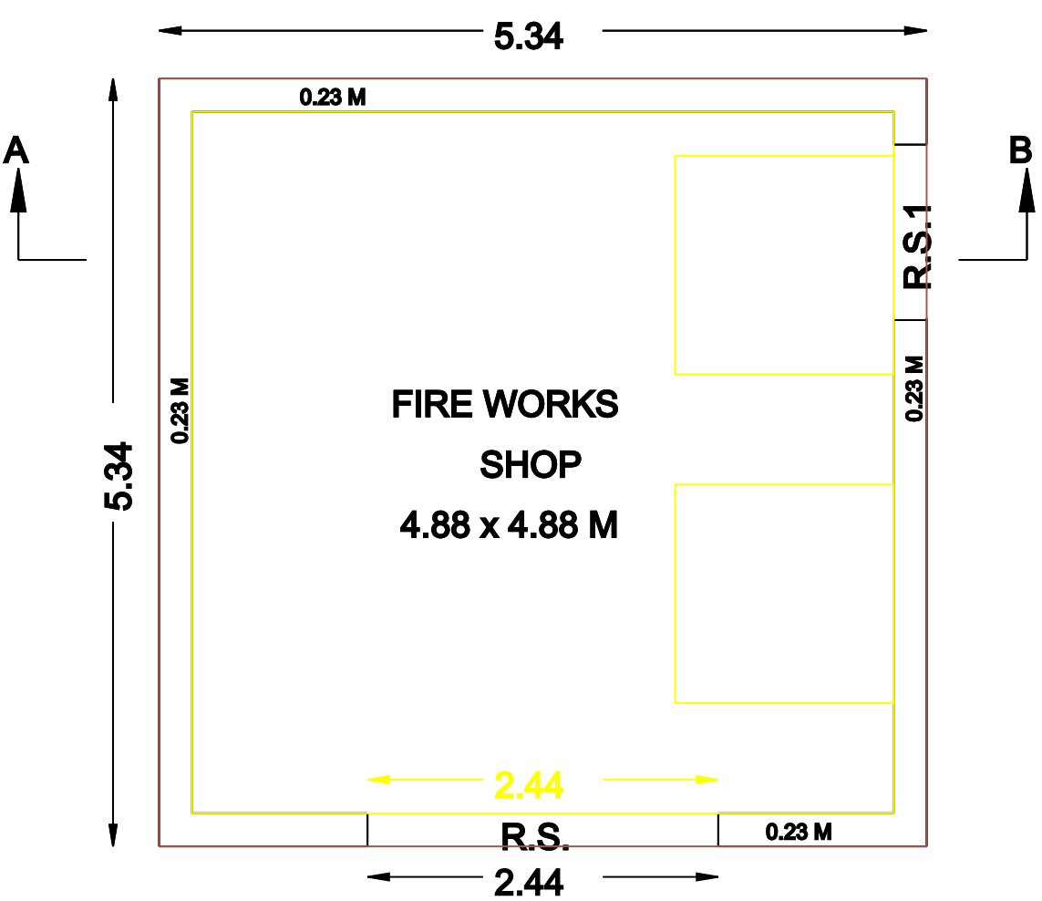
PROPOSED FIRE WORKS SHOP
