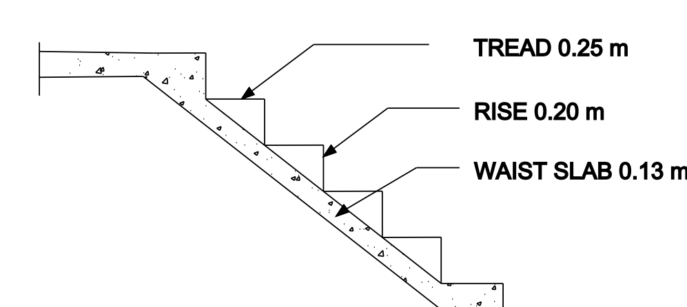
STAIR DETAILS
