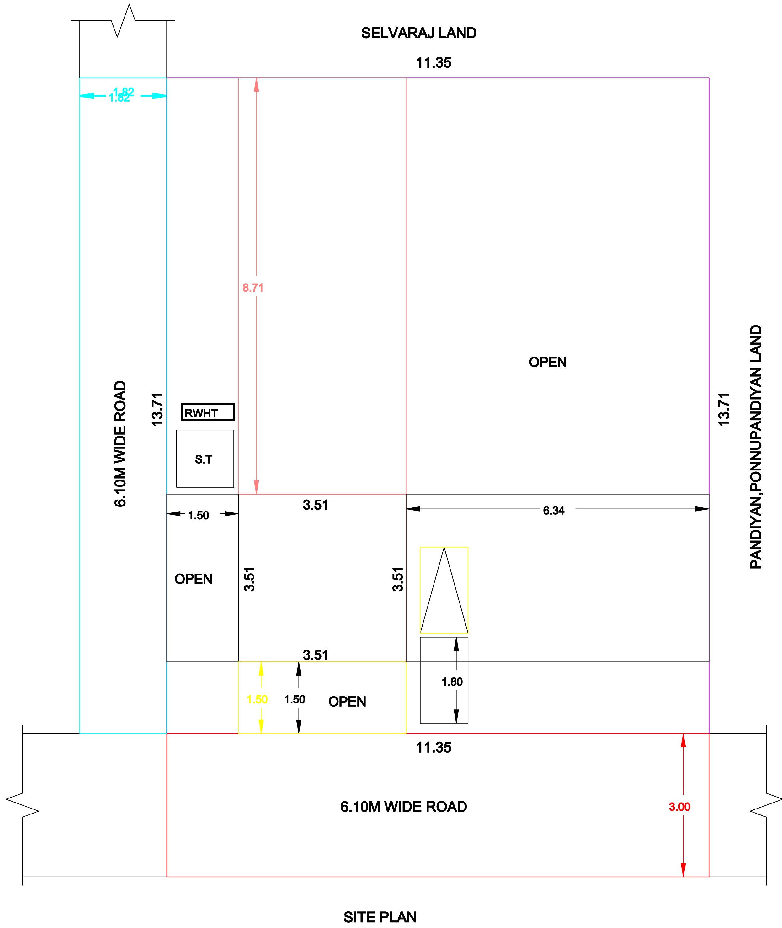
SITE PLAN
