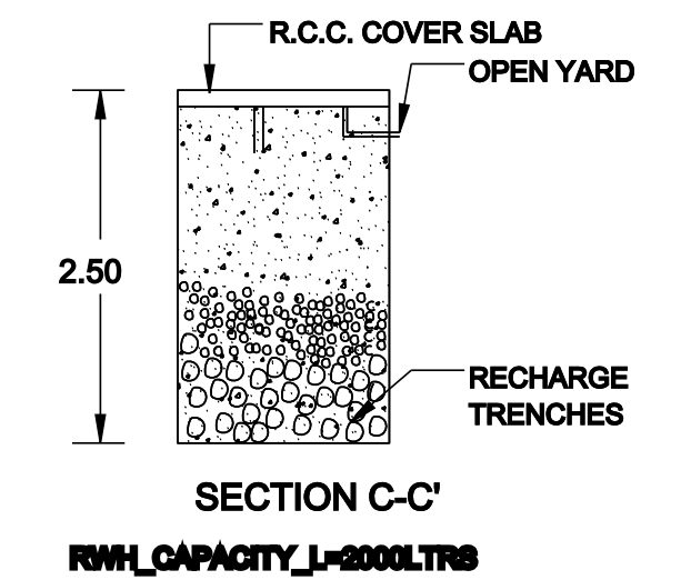
SECTION C-C'
