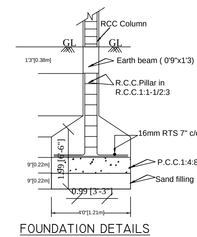
FOUNDATION DETAILS
