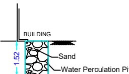
DETAILS OF RAIN WATER PERCOLATION PIT (SCALE 1:100)
