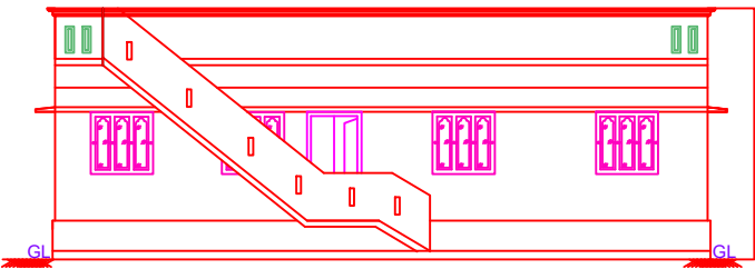
FRONT ELEVATION
