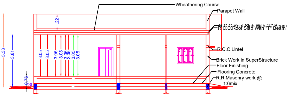
SECTION ON "PQ" SCALE 1:100
