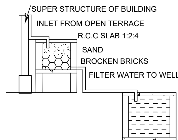
RAINWATER HARVESTING
