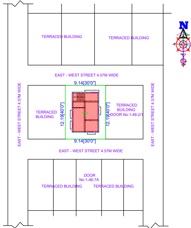
KEY PLAN (AS PER DOCUMENT / SITE)
