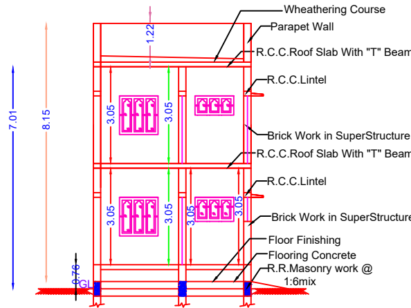
SECTION ON "PQ" SCALE 1:100
