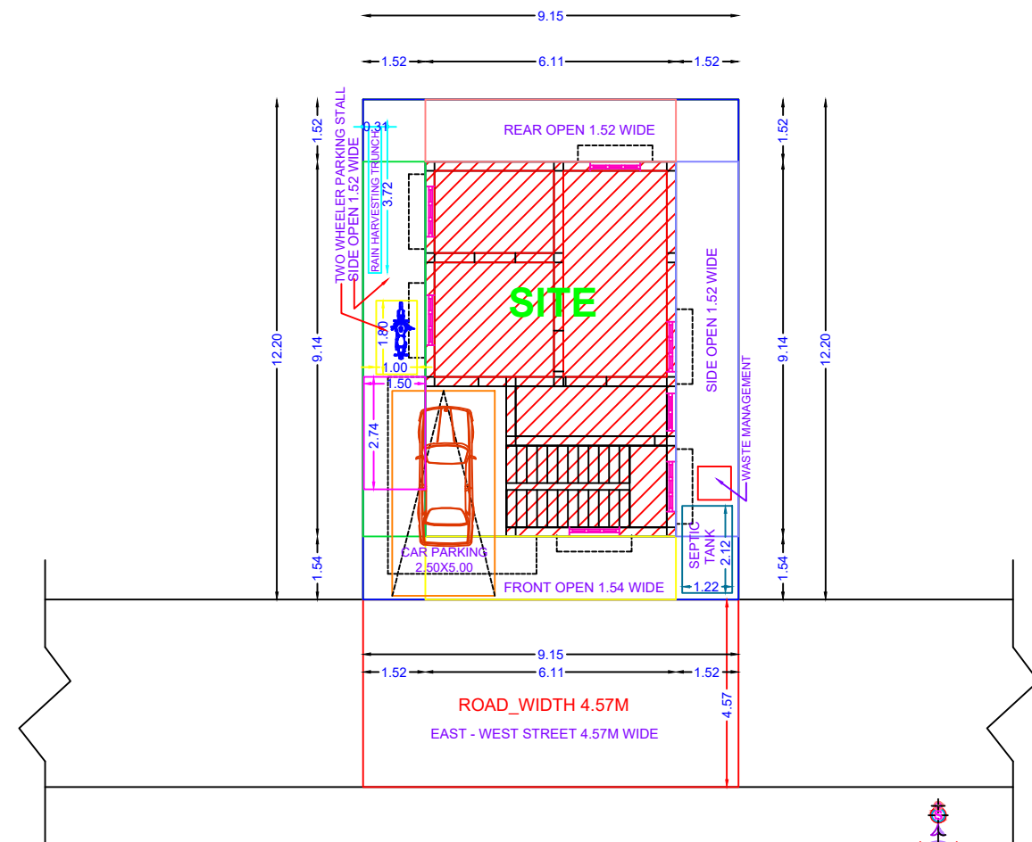
SITE PLAN
