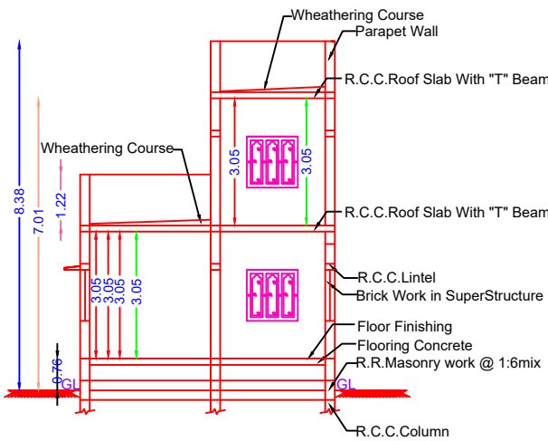
SECTION ON "PQ"
