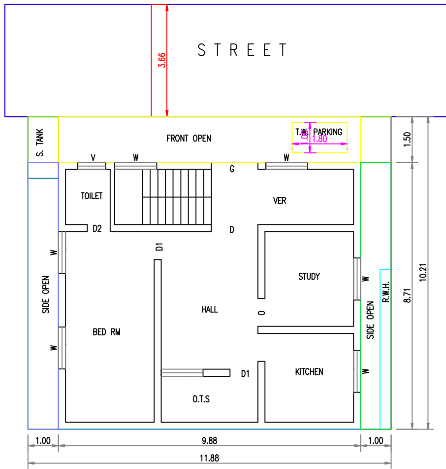
SITE PLAN
