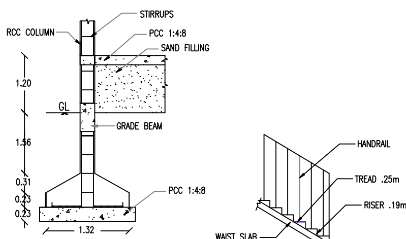
COLUMN DETAILS
