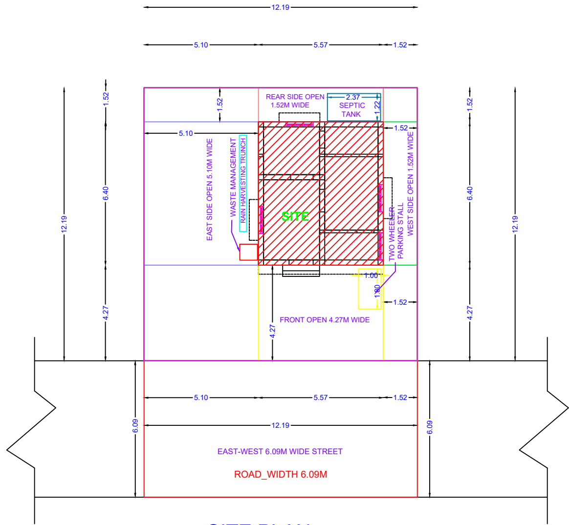
SITE PLAN
