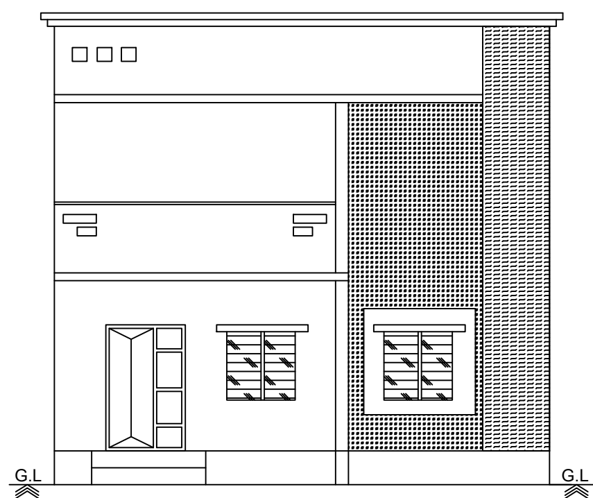
FRONT ELEVATION
