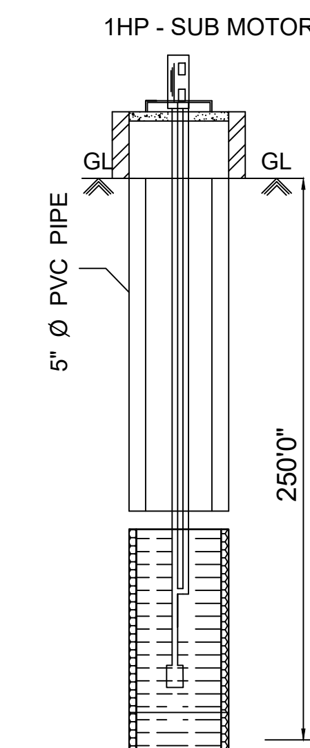
BOREWELL DETAILS
