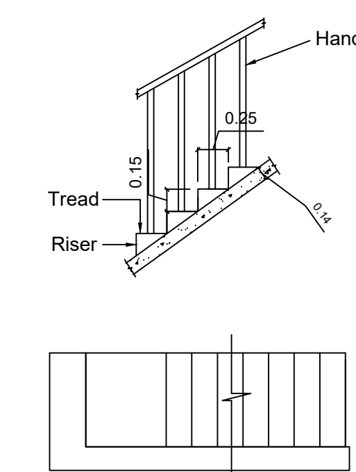
STAIRCASE DETAIL
