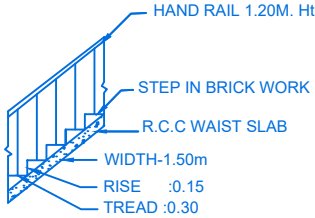
STAIR DETAIL
