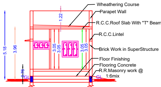
SECTION ON "PQ" SCALE 1:100
