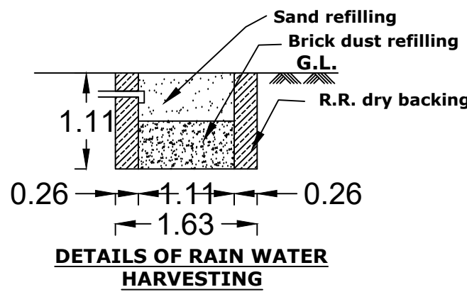
DETAILS OF RAIN WATER HARVESTING
