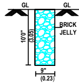
PERCOLATION PIT
