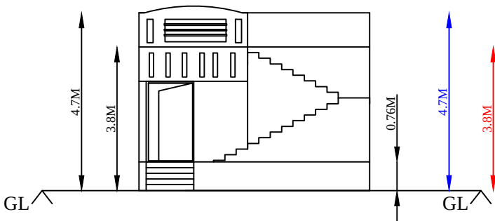
FRONT ELEVATION
