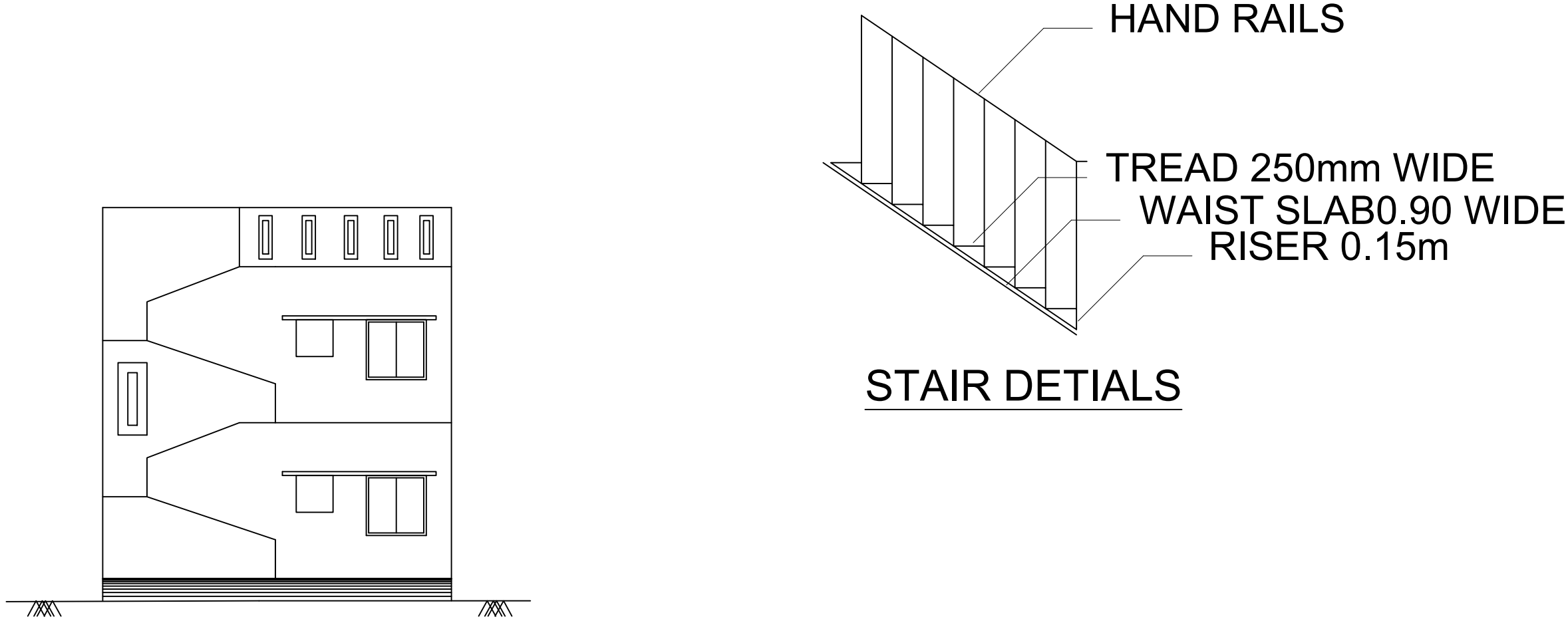
FRONT ELEVATION
