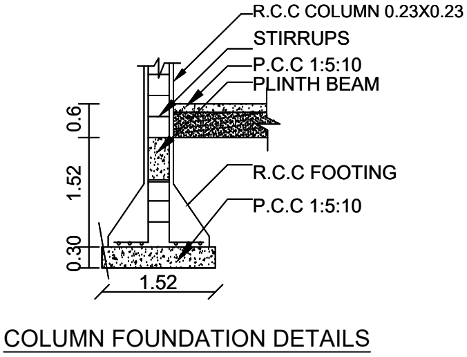
COLUMN FOUNDATION DETAILS
