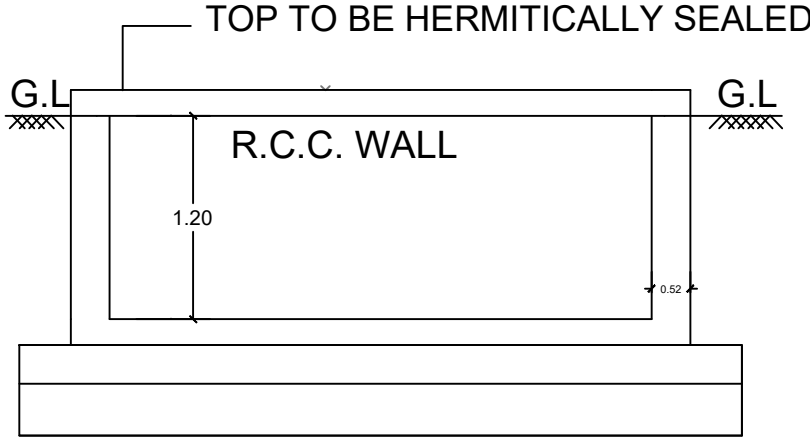
RWH_CAPACITY_L = 2000 RWH SECTION
