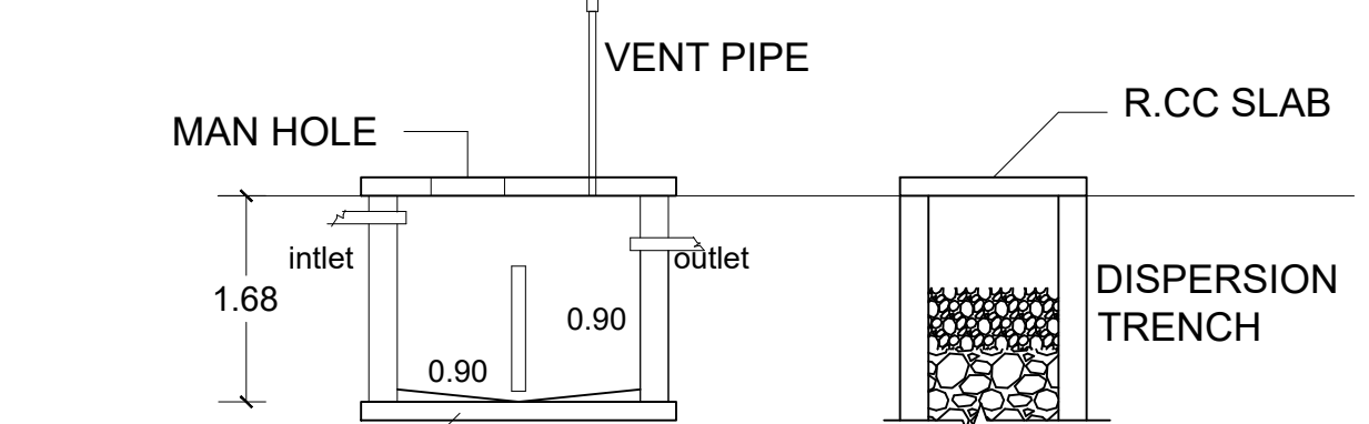
SEPTIC TANK SECTION
