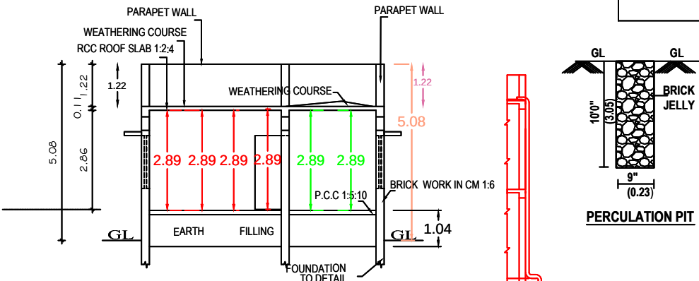
SECTION "A-B"
