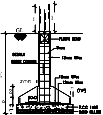
FOUNDATION DETAILS
