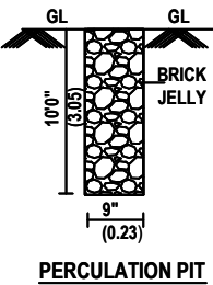
PERCOLATION PIT
