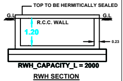
RWH SECTION
