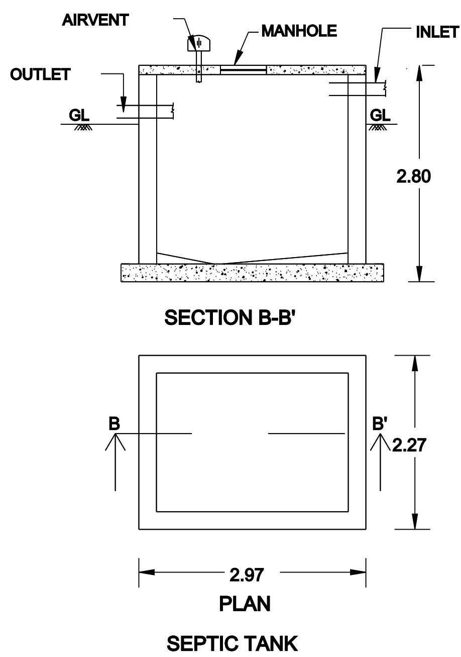
SEPTIC TANK
