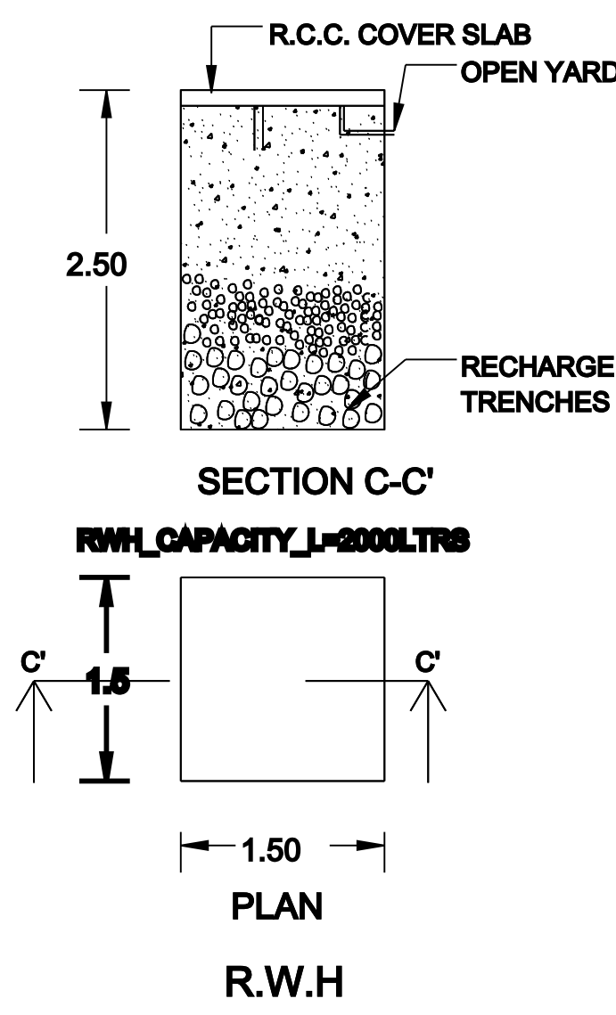
PLAN
