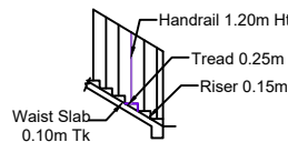
DETAILS OF STAIR CASE (SCALE 1:100)
